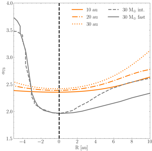
Figure 7. Spectral indices calculated from the synthetic images in Band 3 and 7, for the three different transition disc models, compared with the intermediate and fast migration case from Nazari et al. (2019), shifted to be centred at the cavity edge and zoomed in the cavity region.
