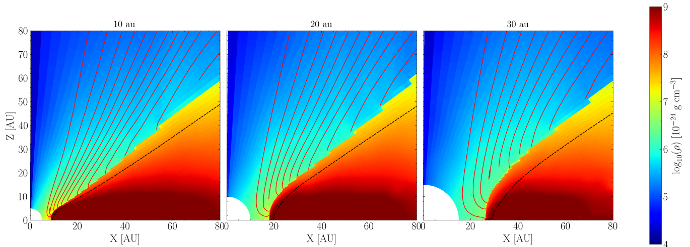
Figure 1. Gas density distributions for the different runs in the inner 80 au. The black dashed line show the maximum penetration depth of X-rays ( N_X = 2 \cdot 10^{22} pp \text{cm}^{-2} ), while the red lines show gas streamlines in the wind every 8% of the cumulative mass-loss rate.
