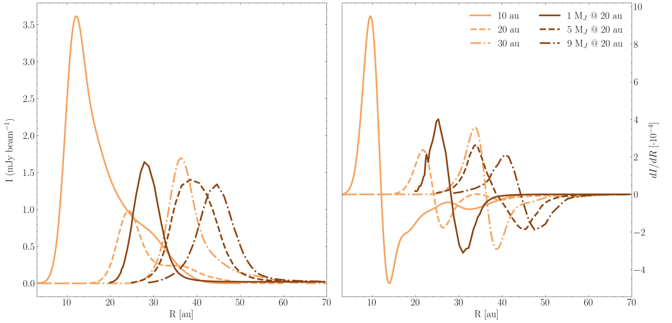
Figure 6. Panel a: radial intensity profile in Band 7 for this work in orange and from de Juan Ovelar et al. (2016); Facchini et al. (2018) for a 1, 5, and 9 M_J mass planet in brown. Panel b: gradients of the intensity curves. We adopted a 0.03'' resolution beam and a distance of 150 pc for direct comparison.
