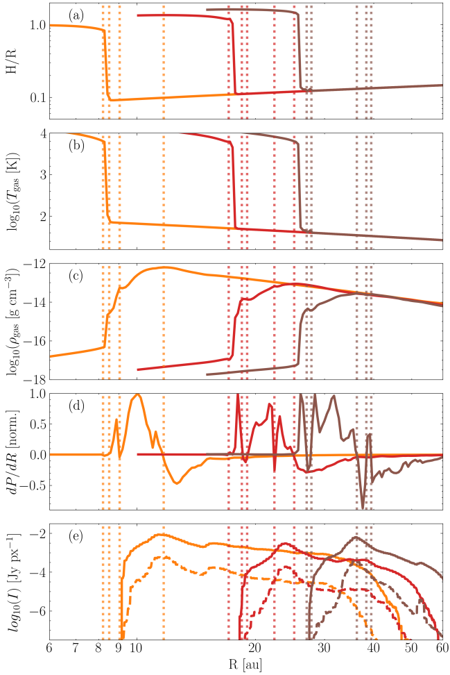
Figure 2. Panel a: disc scale height radial profile. Panel b: gas temperature radial profile. Panel c: mid-plane gas density radial profile. Panel d: normalized mid-plane pressure gradient. Panel e: radial profile of the continuum intensity in Band 3 (solid) and 7 (dashed dotted line). With dotted vertical lines the location of zero pressure gradient are reported. In all panels the orange, red, and brown lines represent the 10, 20, and 30 au cavity models respectively.
