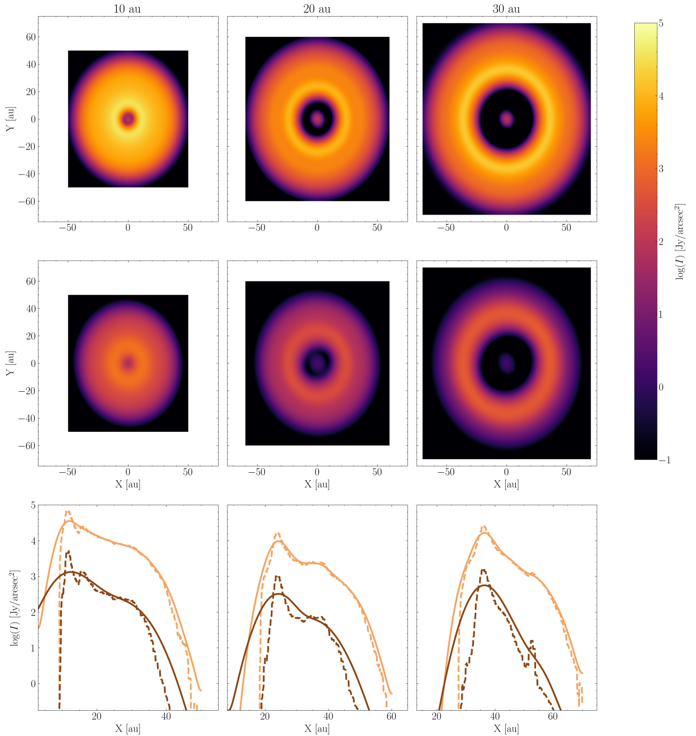
Figure 5. Dust continuum emission in Band 7 (top panel) and 3 (middle panel) convolved with a realistic ALMA beam size for the 10, 20, and 30 au transition discs. The convolution with the beam size blurs the features seen in Figure 4. In the bottom panel the radial profiles are shown for a direct comparison between Band 7 (in orange) and Band 3 (in brown) and the convolved (solid lines) and unconvolved (dashed lines) intensities.
