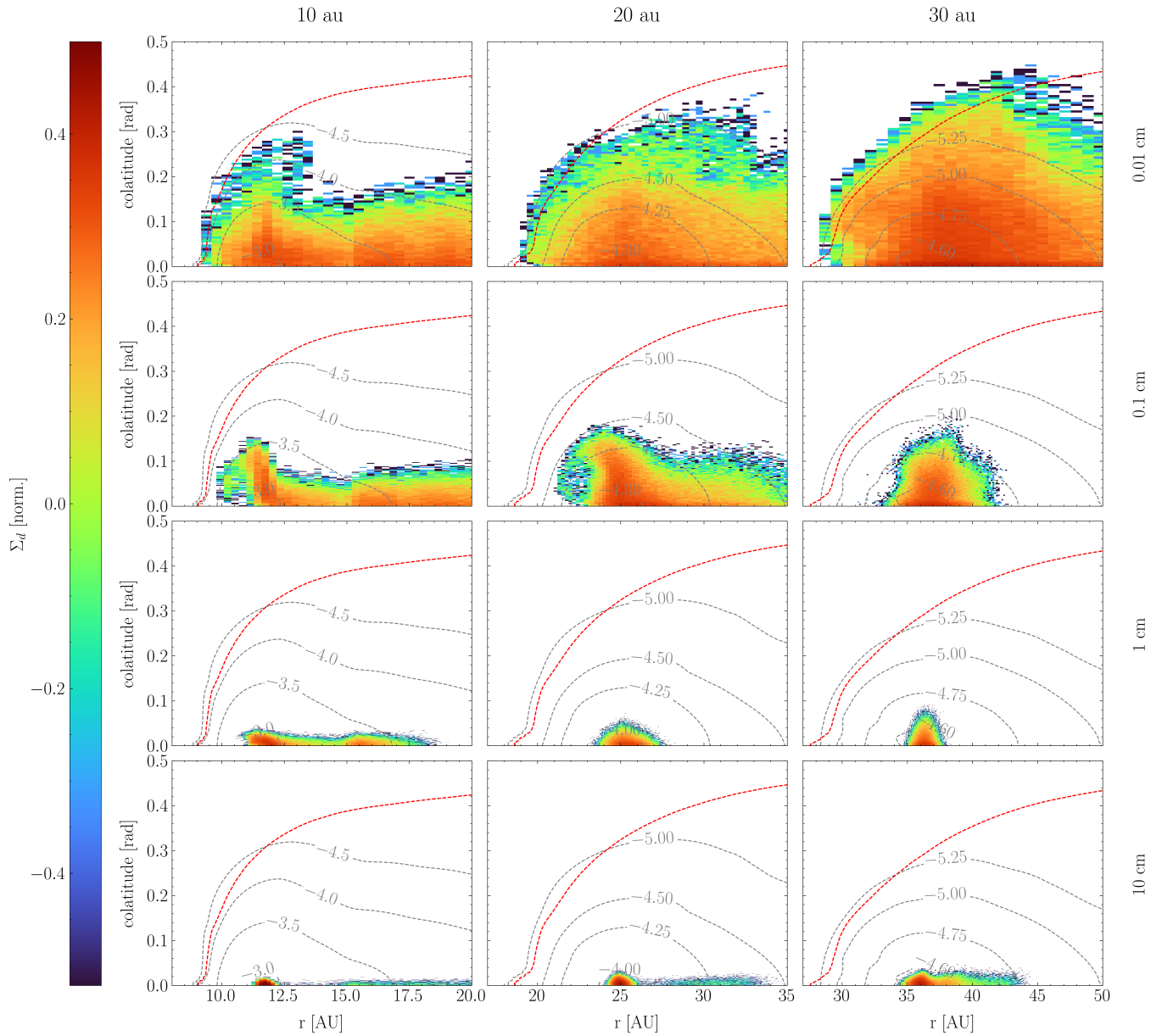
Figure 3. Dust (normalized) density distributions for the four dust particles modelled and the different cavity edges. The red dashed line show the maximum penetration depth of X-rays ( N_X = 2 \cdot 10^{22} pp \text{cm}^{-2} ), while the dashed black lines show the isocontours of gas pressure in log scale. The snapshot is taken after 1,500 yr of dust insertion.
