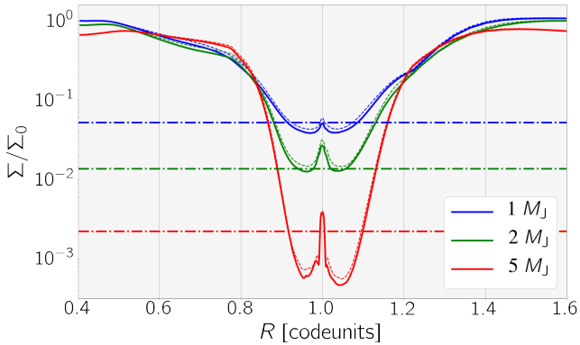
Figure 3. Surface density radial profile for 1, 2 and 5 M_J planets after the simulations reach a steady-state, shown as solid lines. The dash-dot lines are the respective predicted gap-depths, derived from an analytical model for gaps in protoplanetary discs (Duffell 2015). The dashed lines represent the surface density after 20 orbits. A value of 1 in radial code units is equivalent to 5.2 AU.
